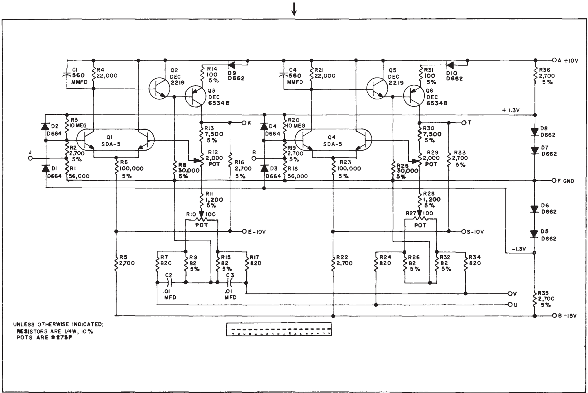
A202-0-1 Two Analog Preamplifiers
