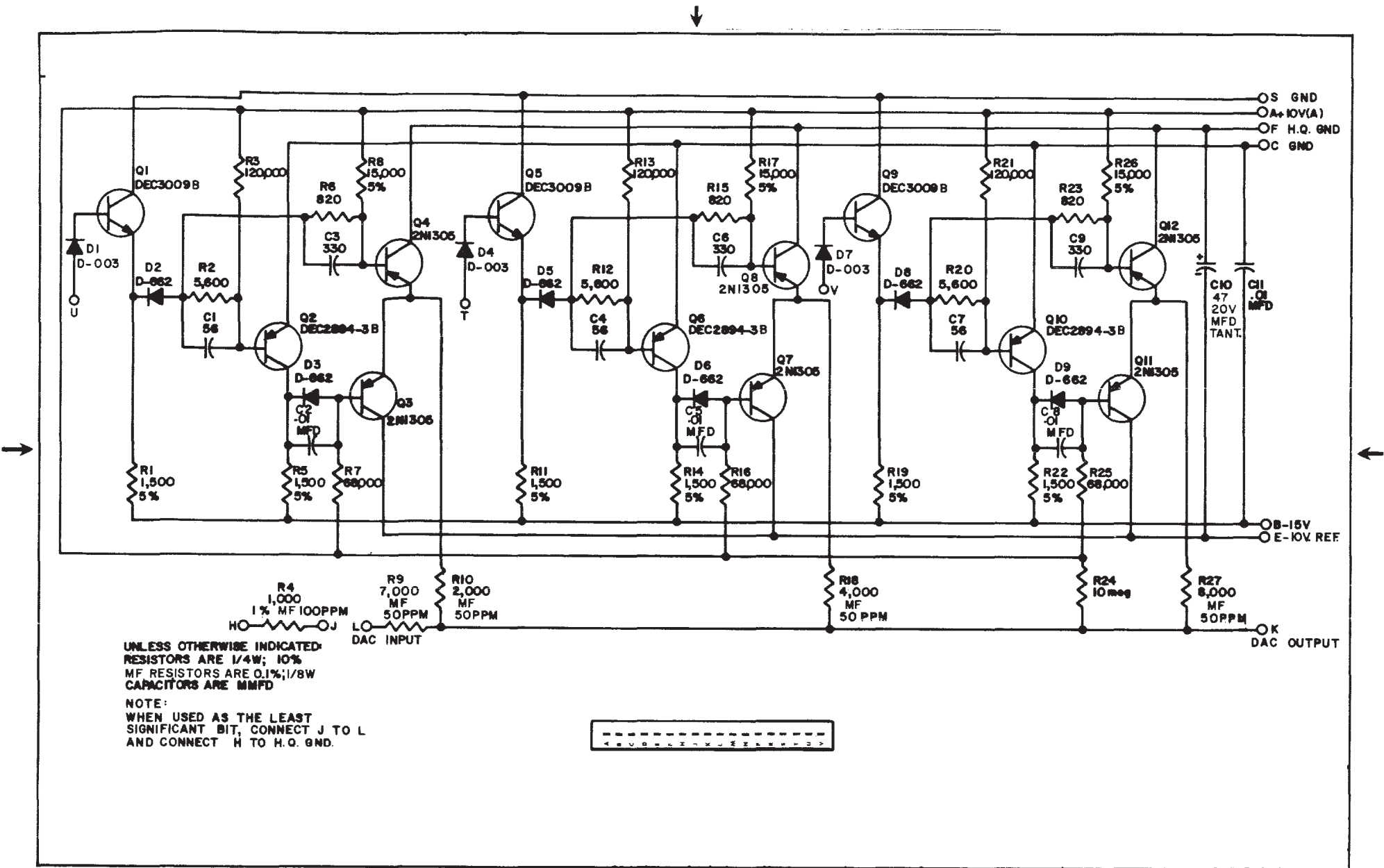
A601-0-1 3 Bit DAC
