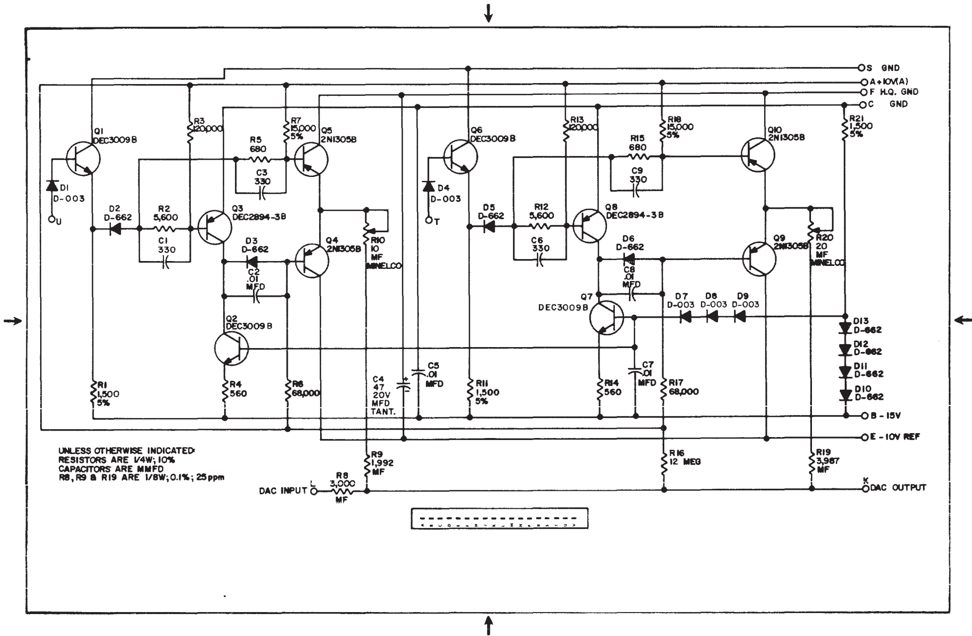
A604-0-1 2 Bit DAC
