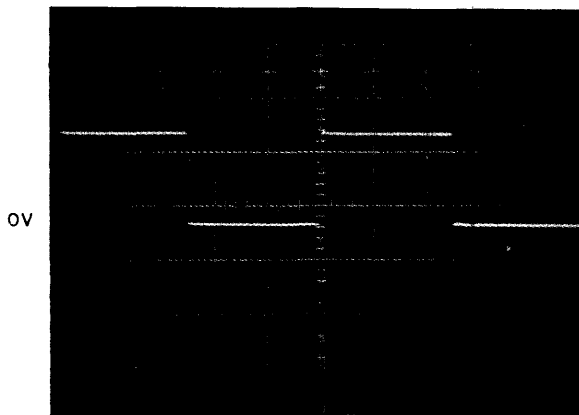
Q10 Emitter to Base Voltage
