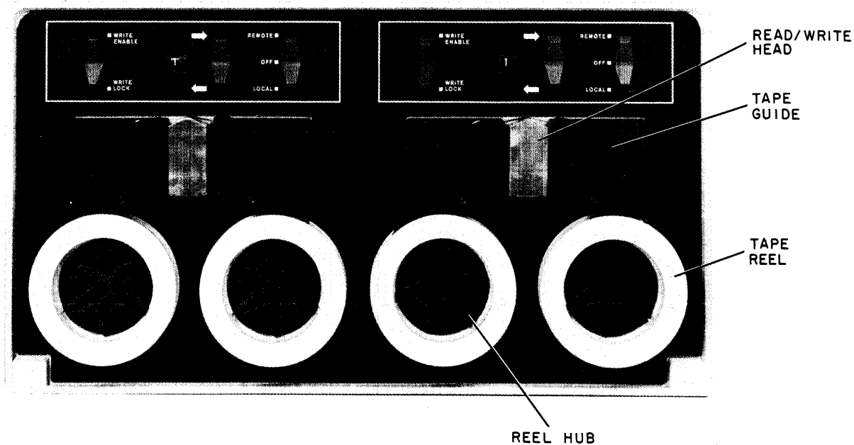
A. Mounting Panel (closed)
