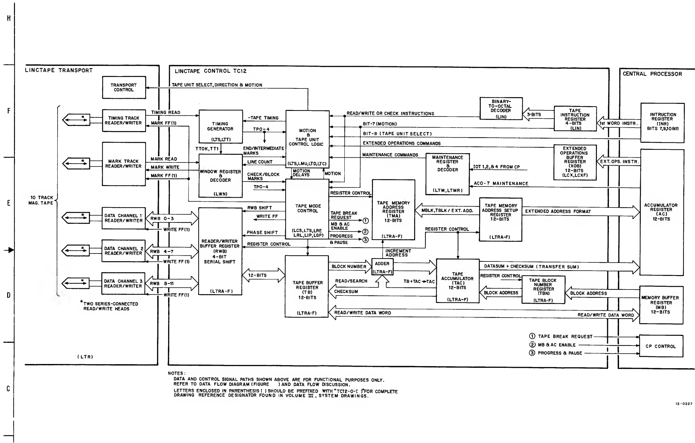
Figure 6-9 LINCtape Overall Block Diagram
