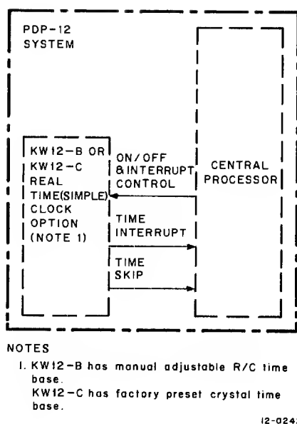
Figure 7-14 KW12-B and KW12-C Simple Clocks, PDP-12 System Functional Relationships
