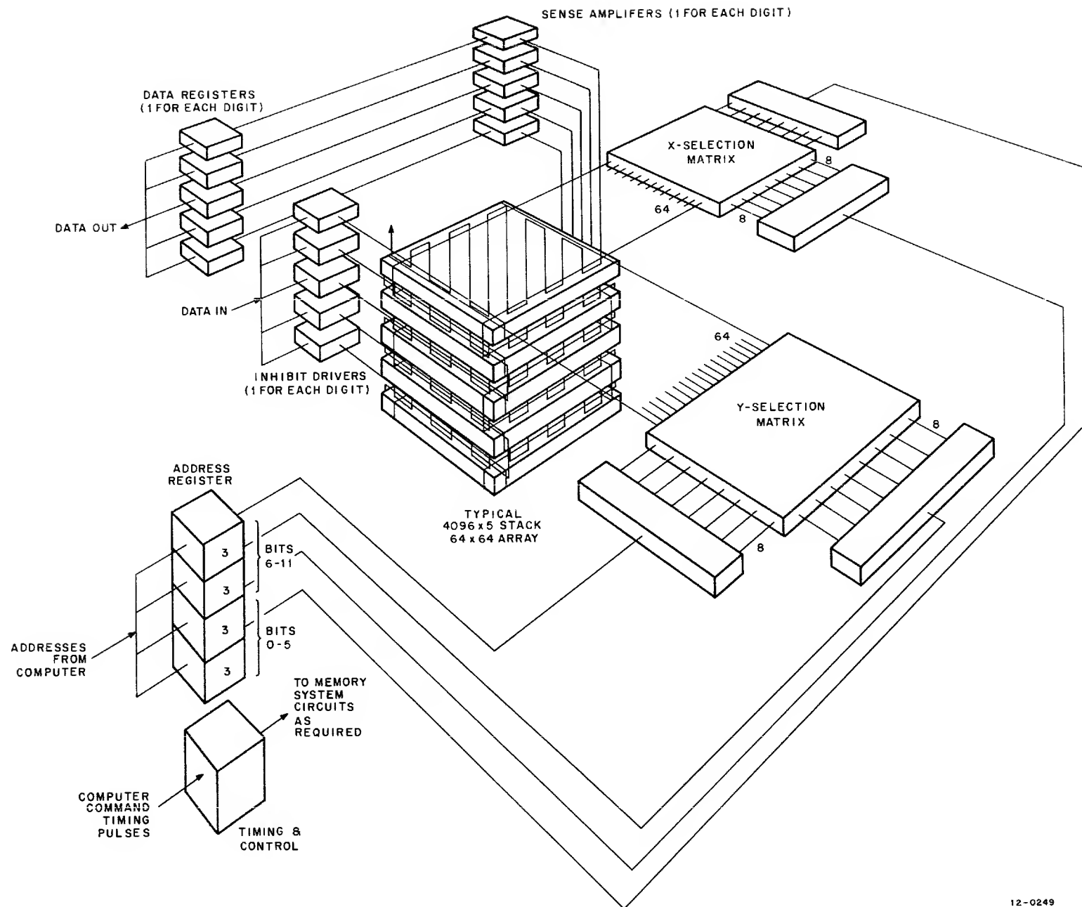
Figure 2-1 Elements of PDP-12 Core Memory
