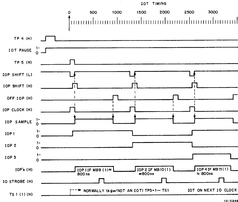
Figure I-10 IOT Timing
