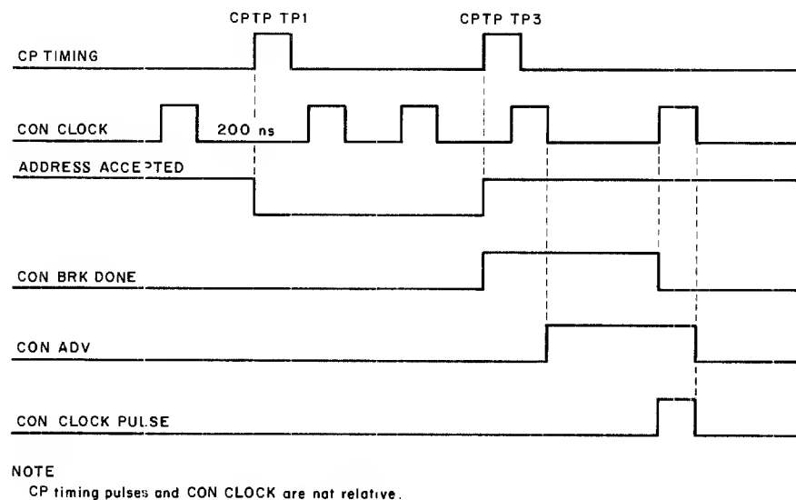
Figure 7-6 Control Timing
