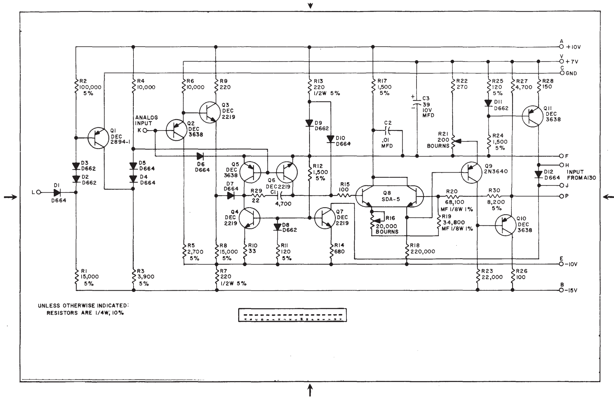
A401-0-1 Sample and Hold
