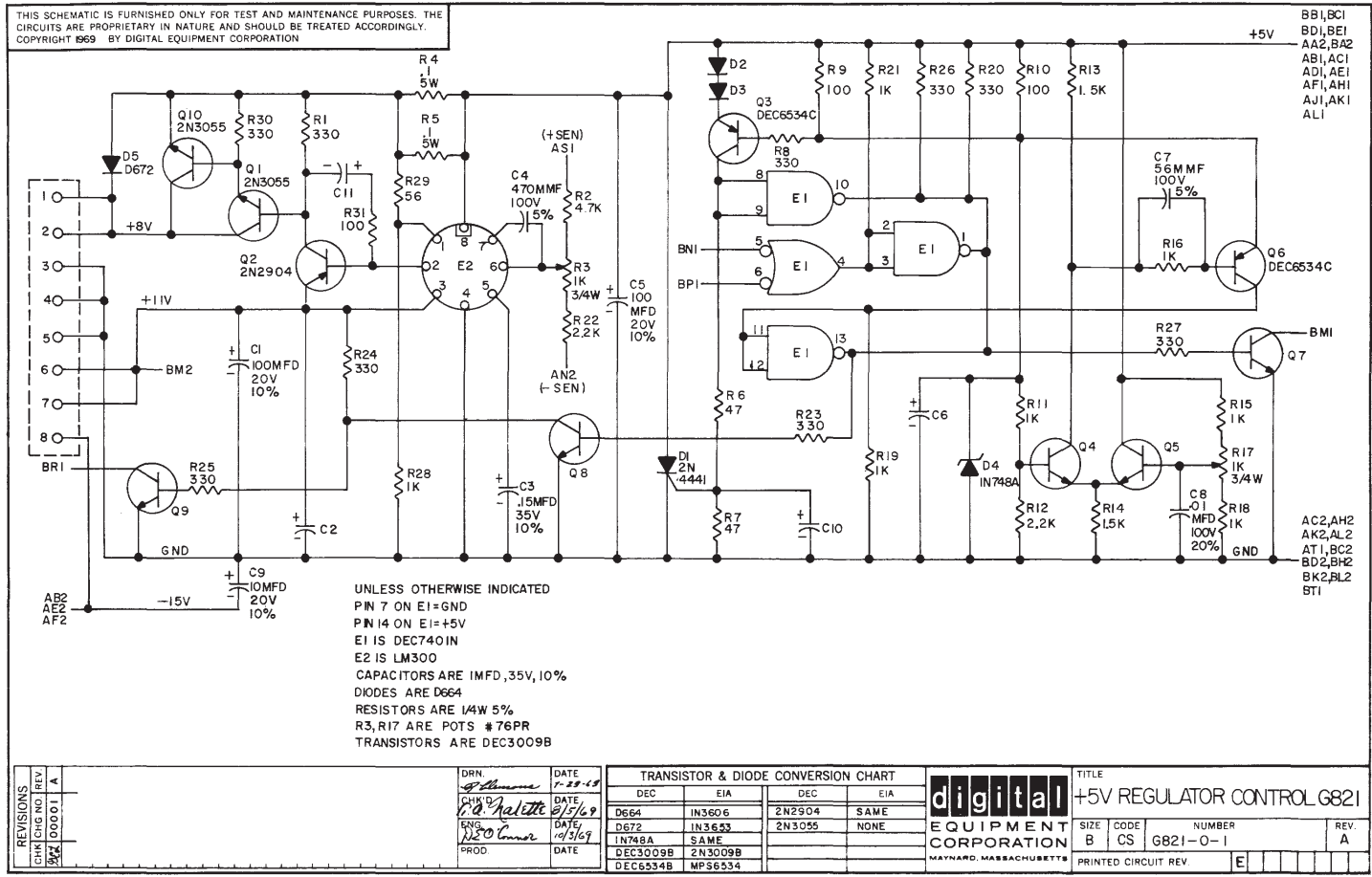
Figure 2-20 G821 +5V Regulator Control, Circuit Schematic
