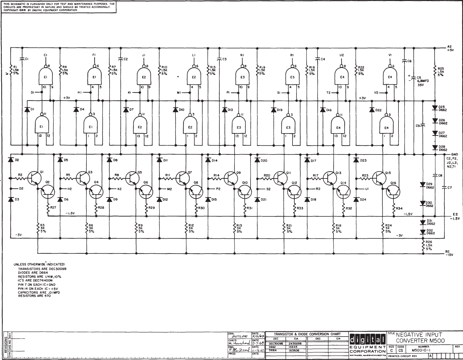
Figure 2-30 M500 Negative Receiver, Circuit Schematic
