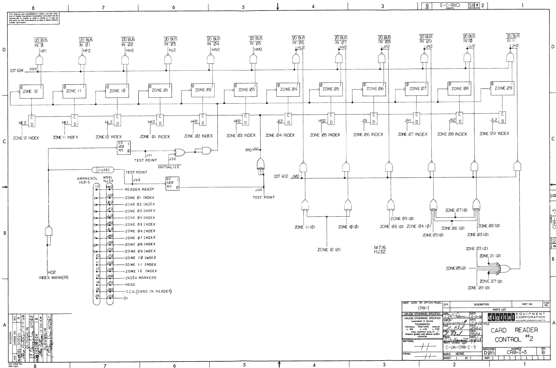
Figure 4-2 CR8/I Logic Schematic (M716)
