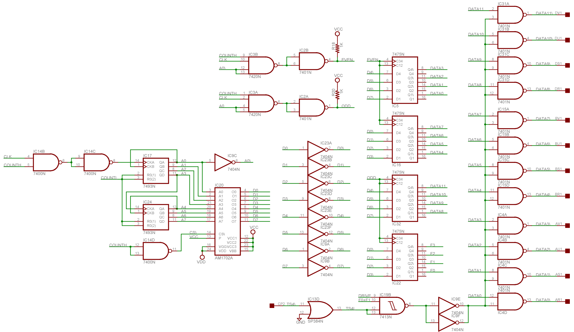
ROM to Data Bus
