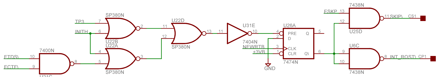
Interrupt Request
