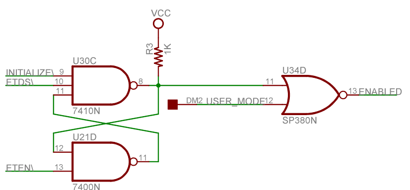
Board Enable
