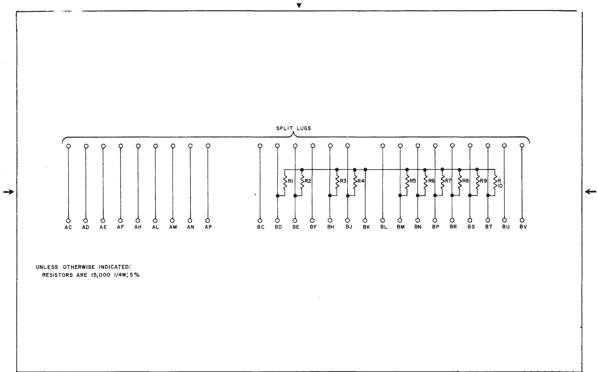
W073-0-1 LINC-8 Tape Cable Connector
