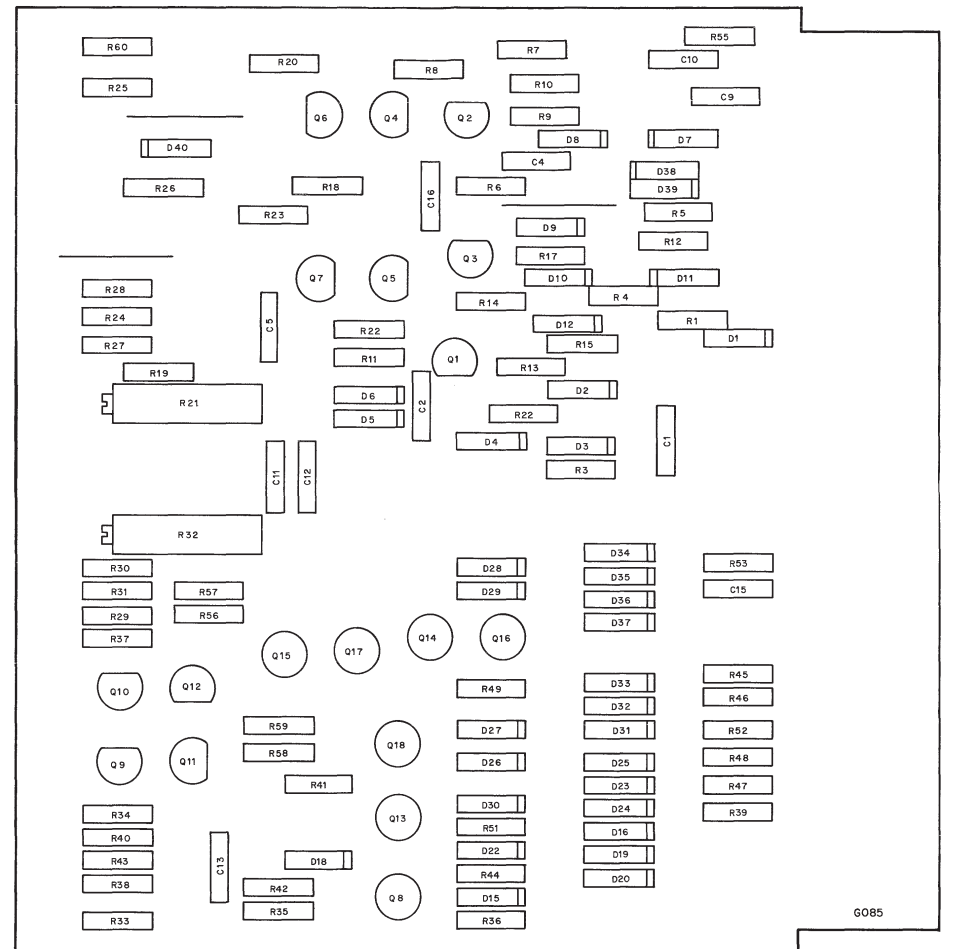
Figure 2-5 Disk Read Amplifier and Slice, Parts Location Diagram
