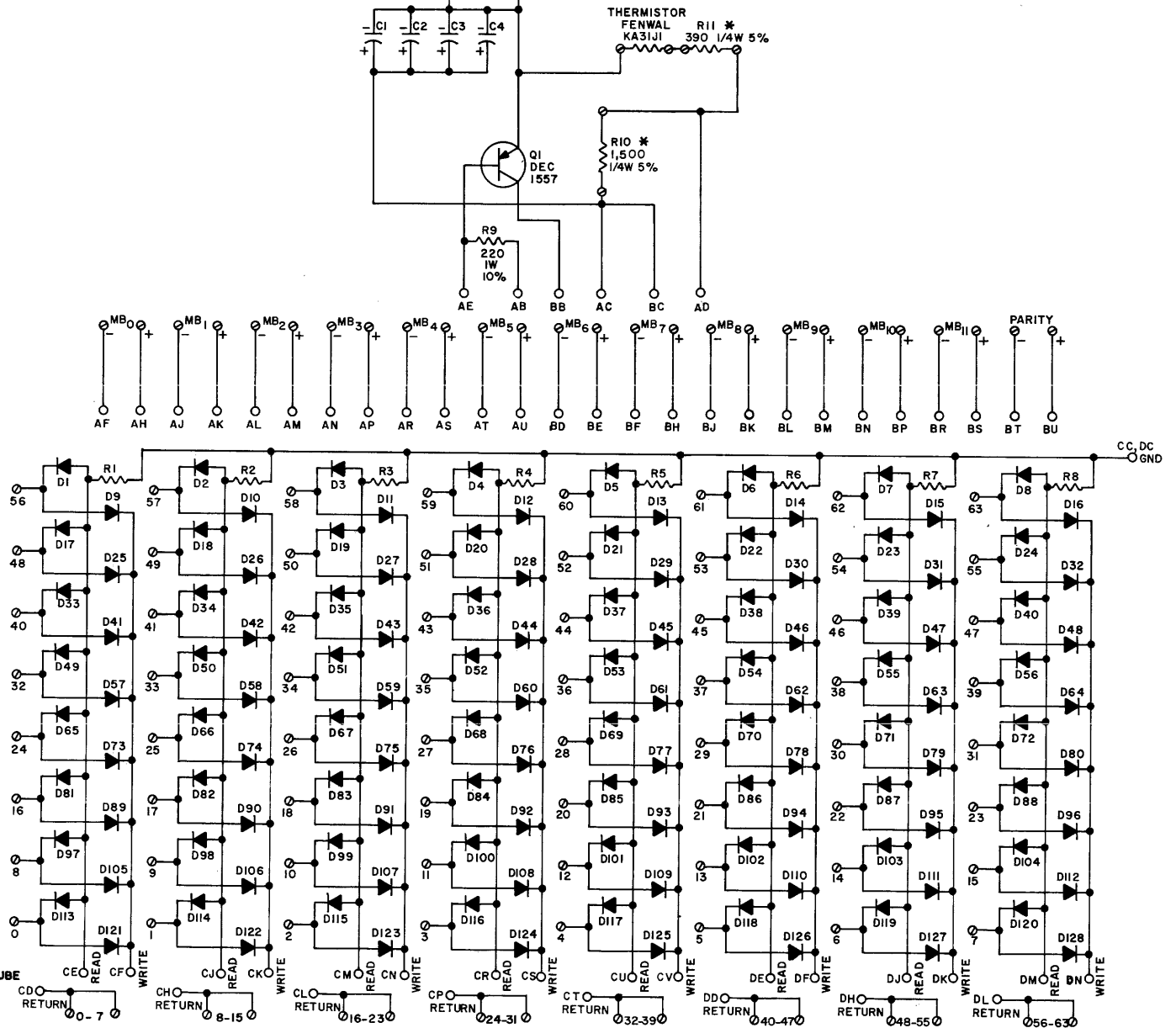
Memory Mounting Board G609
