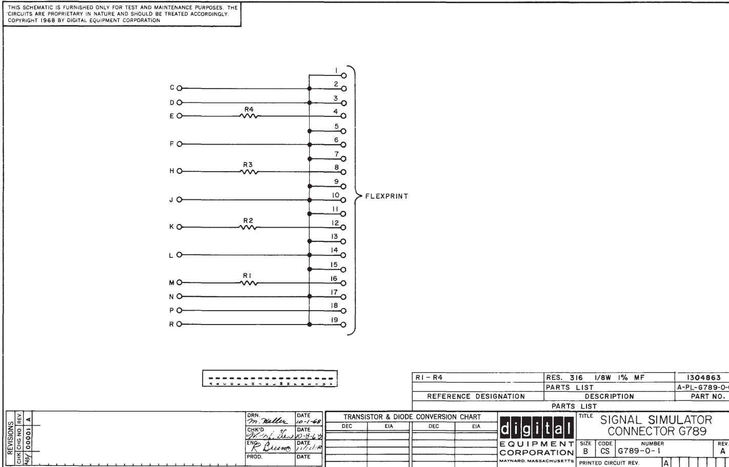
Figure 2-18 G789 Signal Simulator Connector, Circuit Schematic
