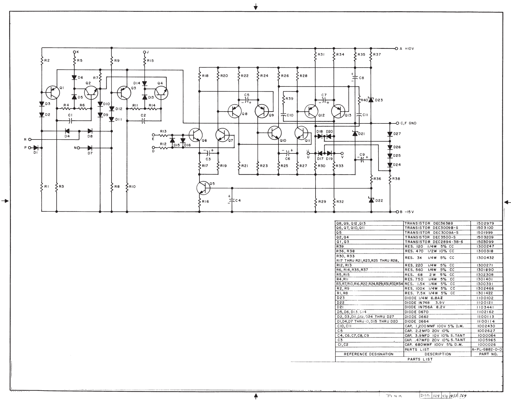
Figure 5-3 G882 Manchester Read/Write Amplifier
