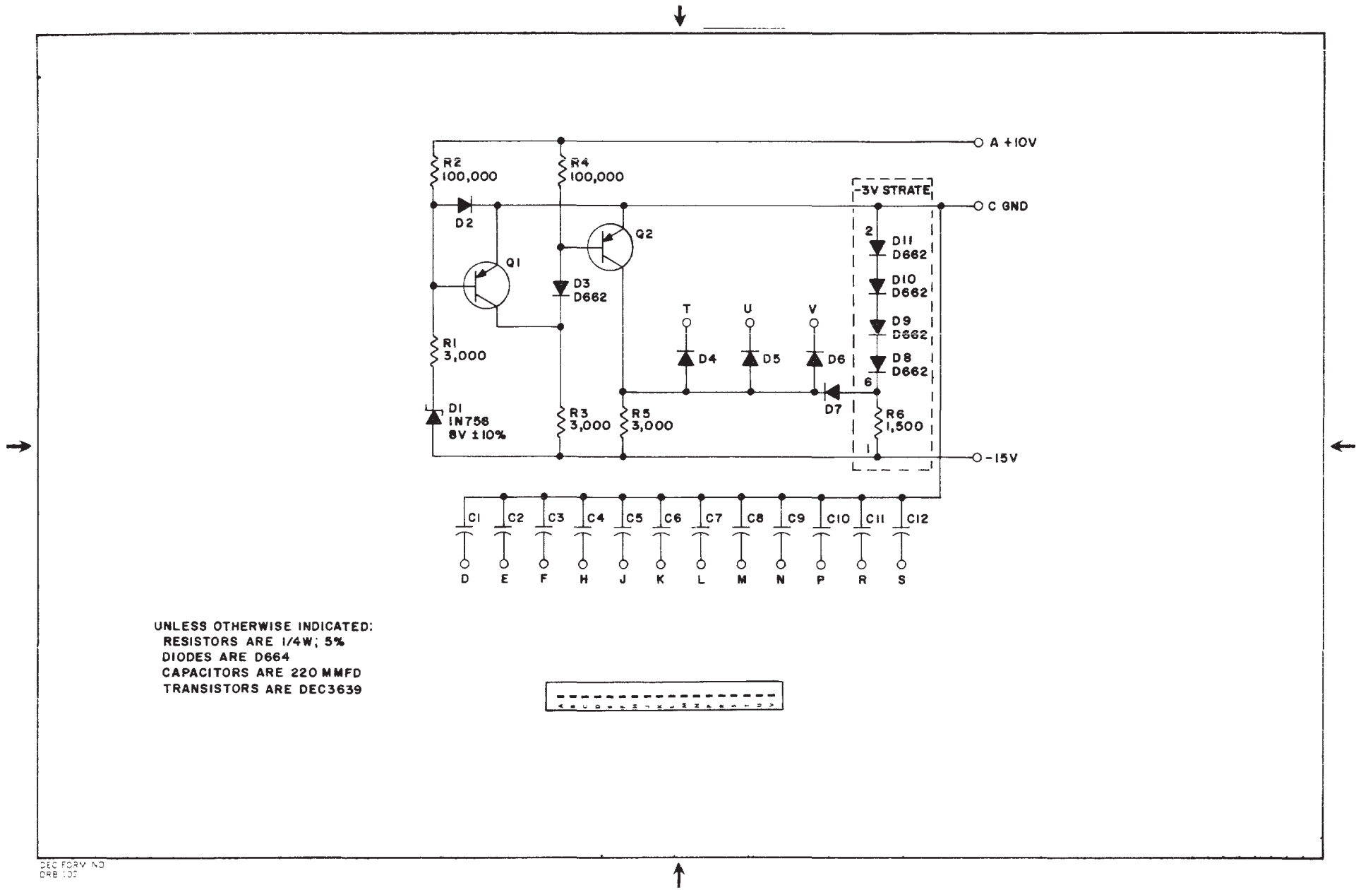
G906-0-1 LINC8 Capacitor and Power Up
