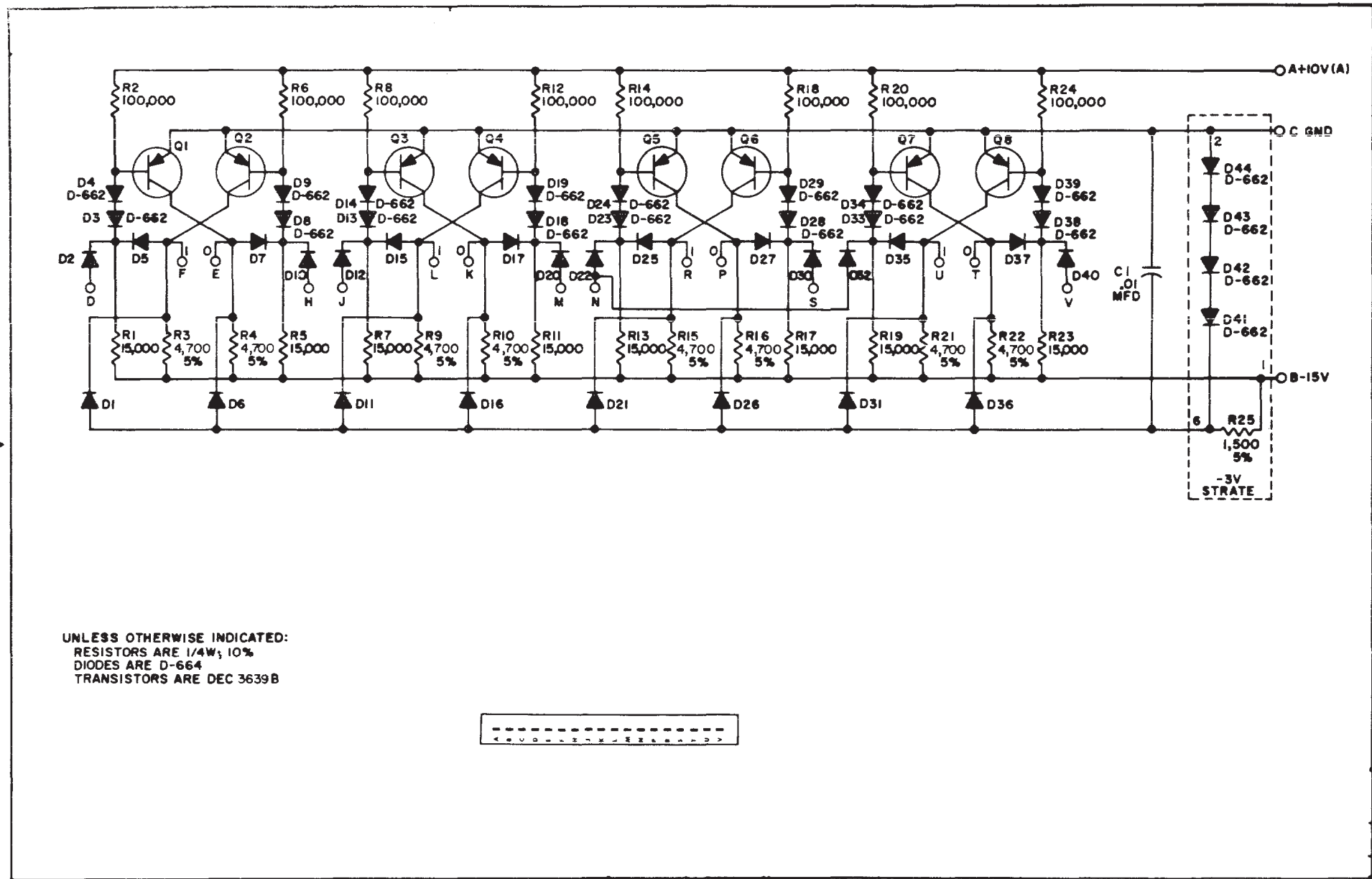
R204-0-1 Quadruple Flip-Flop
