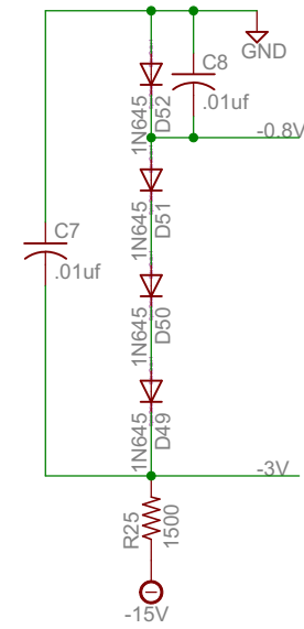
-3V Reference
