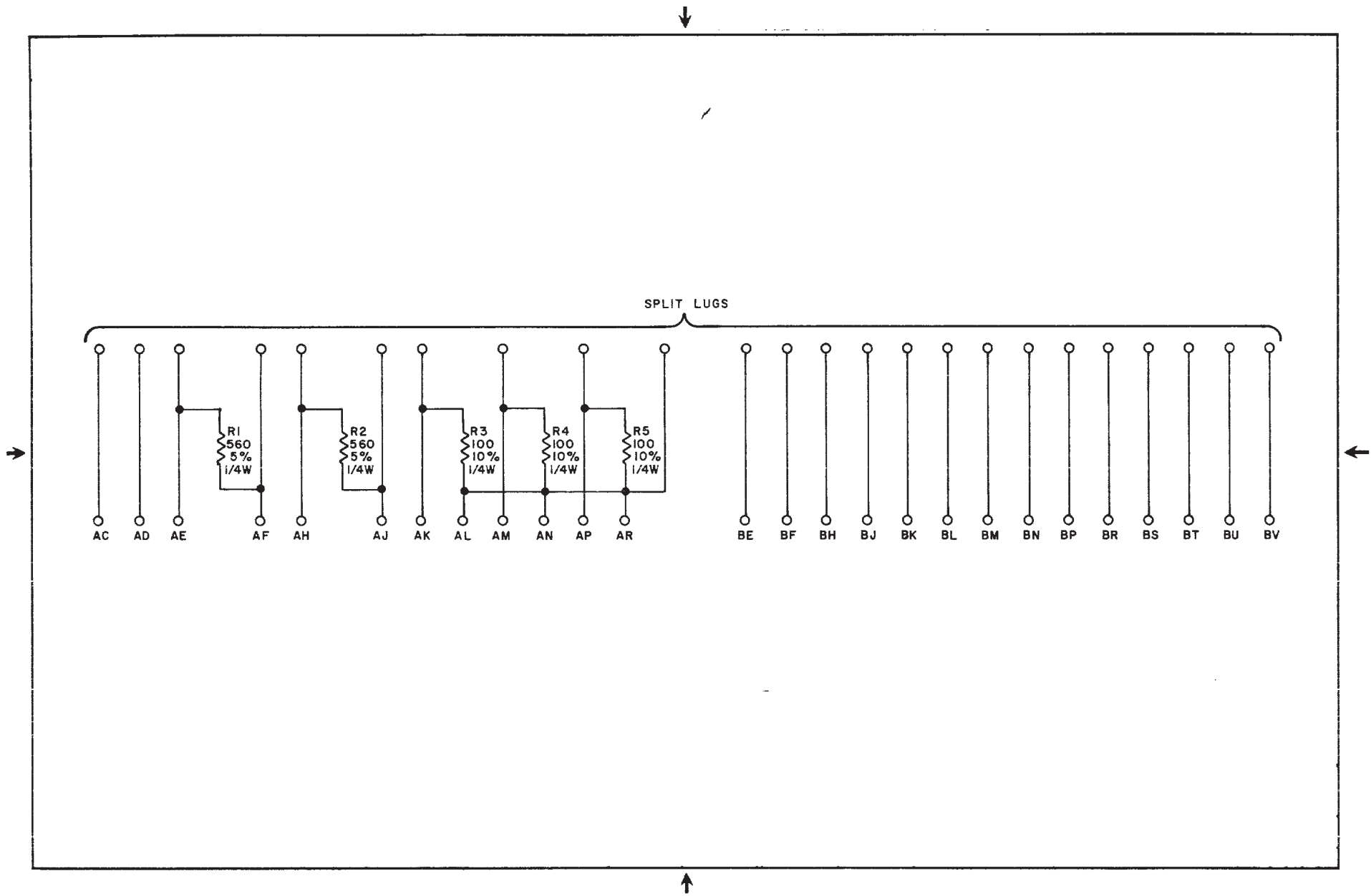
W072-0-1 LINC-8 Scope Cable Connector
