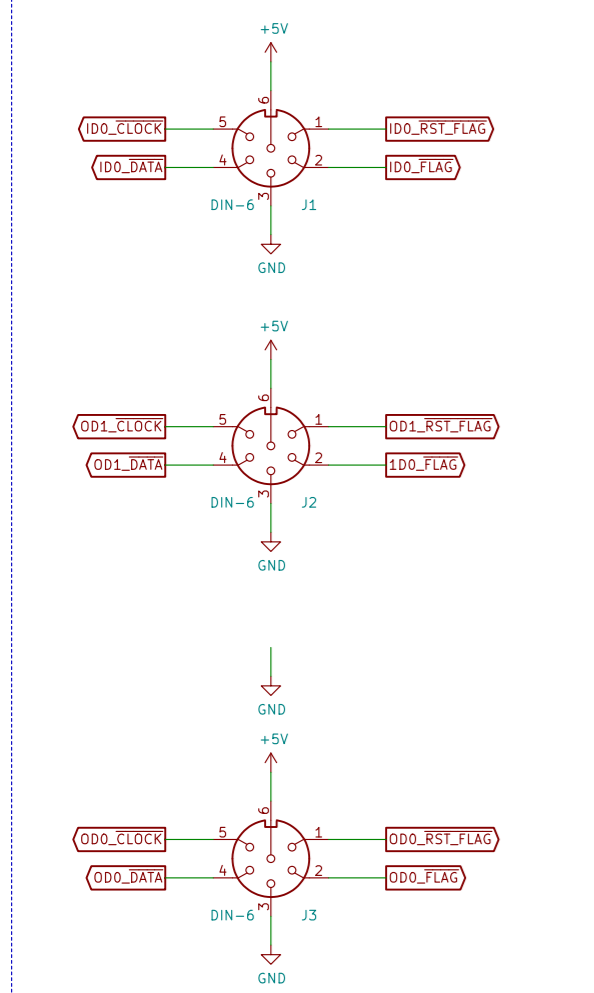
INPUT CONNECTIONS
