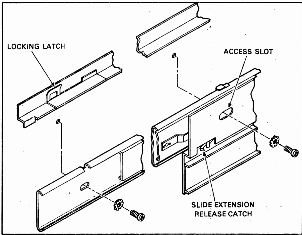
Figure 2-6 Slide Rails
