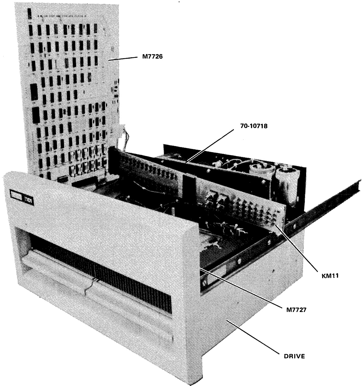
Figure 6-6 KM11 Maintenance Module Inserted
