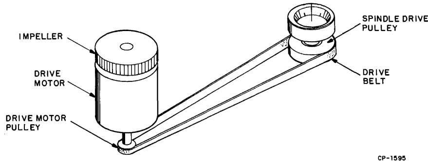
Figure 5-24 Drive Mechanism
