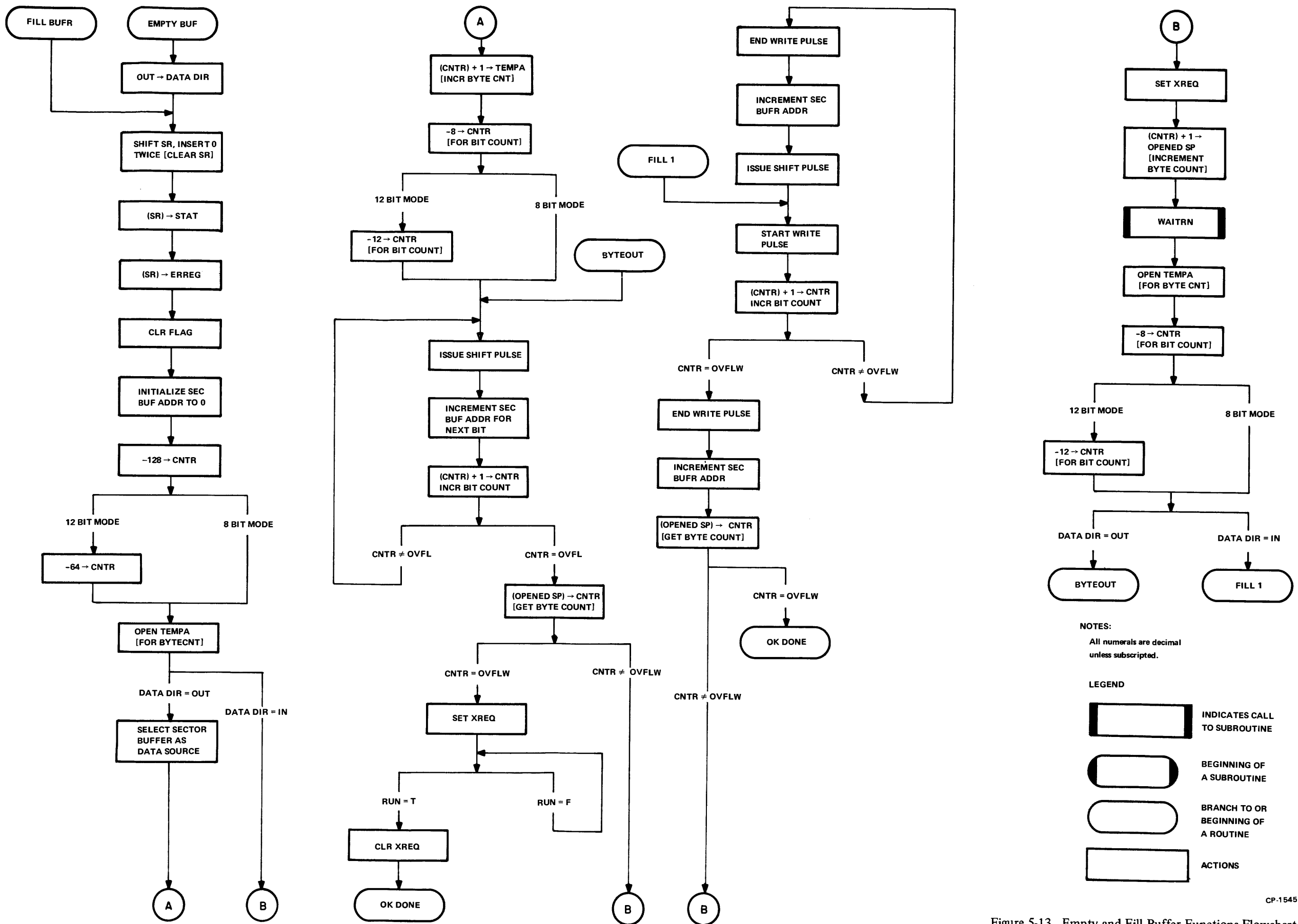
Figure 5-13 Empty and Fill Buffer Functions Flowchart
