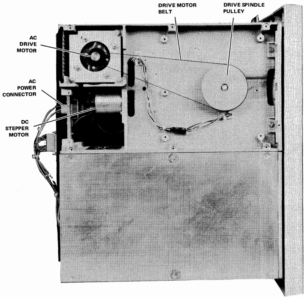
Figure 1-6 Underside View of Drive
