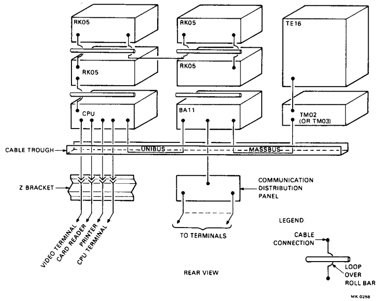
Figure 2-13 Datasystem 534 TE16 Configuration
