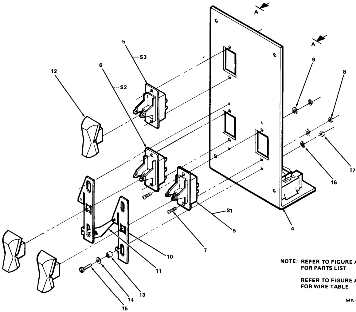
Figure A-8 Initializer Panel (2 of 3)
