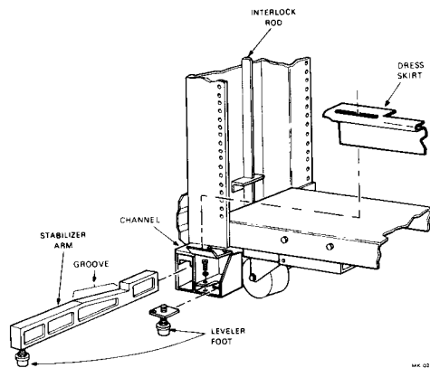
Figure 2-4 Leveler Foot and Stabilizer Arm
