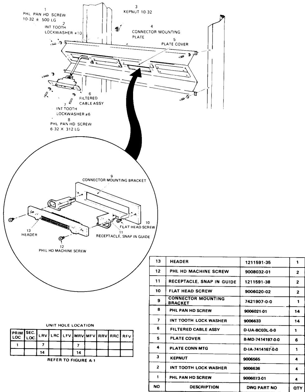
Figure A-18 Connector Mounting Plate (Z Bracket)
