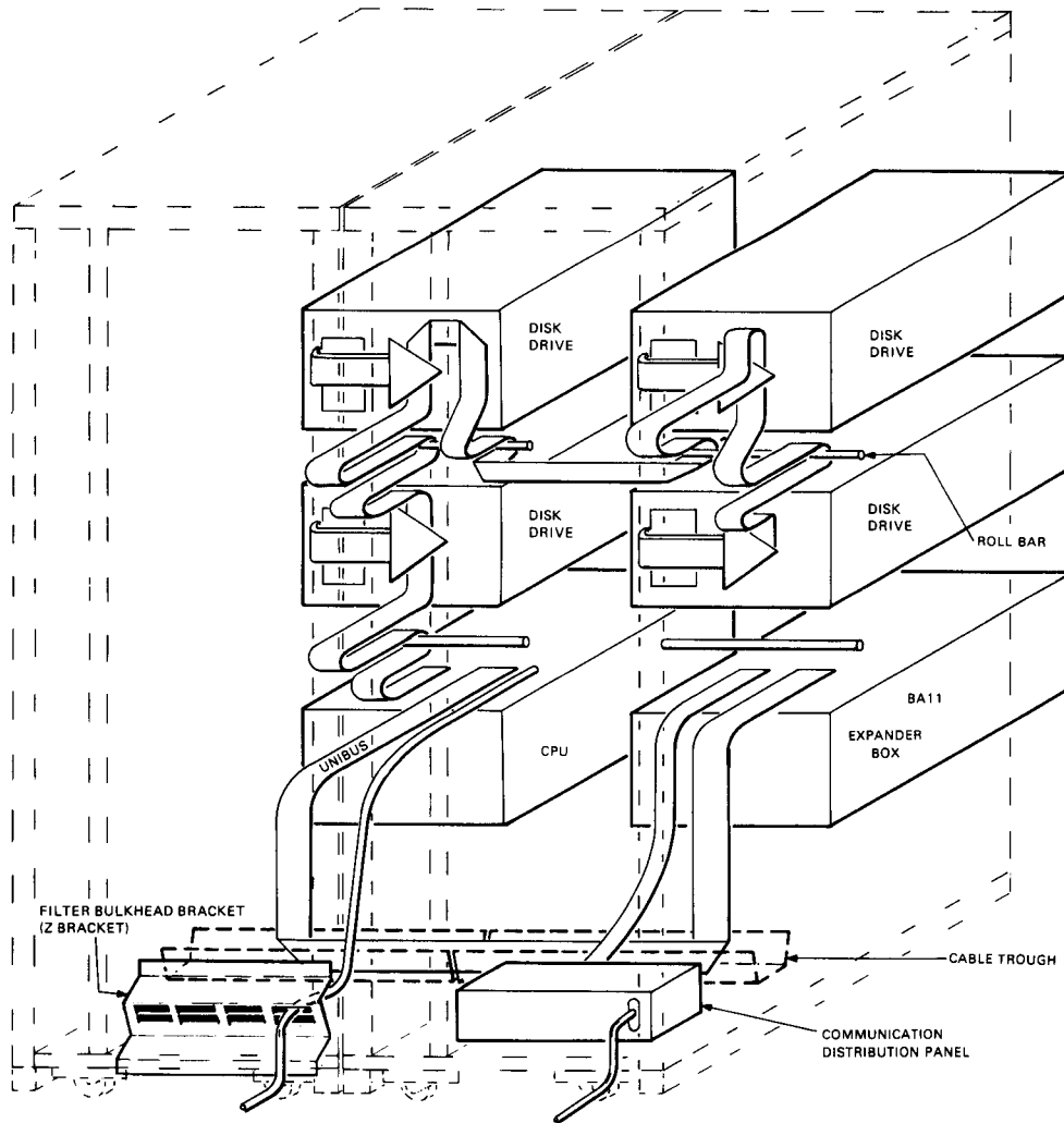
Figure 2-7 Typical Datasystem Cabling Scheme
