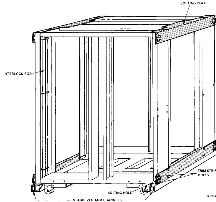
Figure 2-3 Cabinet Frame, Front View
