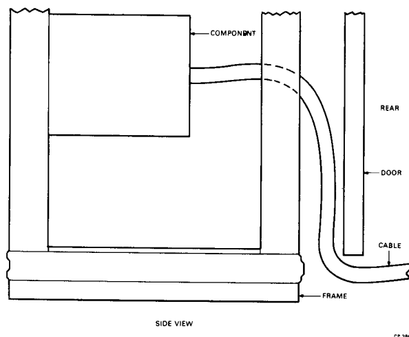
Figure 2-8 Cable Exit From Cabinet
