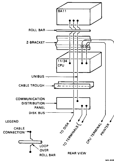
Figure 2-10 Datasystem 530 Cabling Diagram Free-Standing Disk, Basic Configuration
