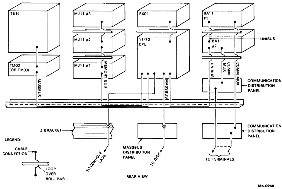
Figure 2-14 Datasystem 570 Cabling Diagram
