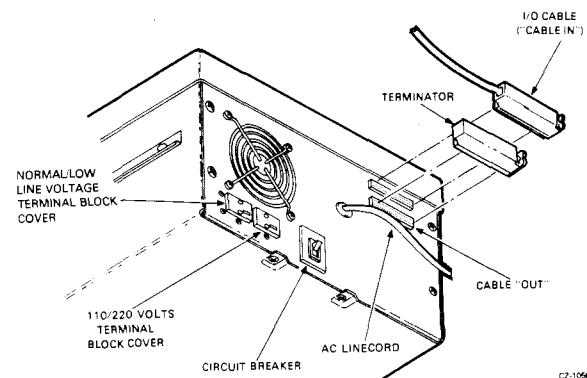
Figure 2-8 Rear View
