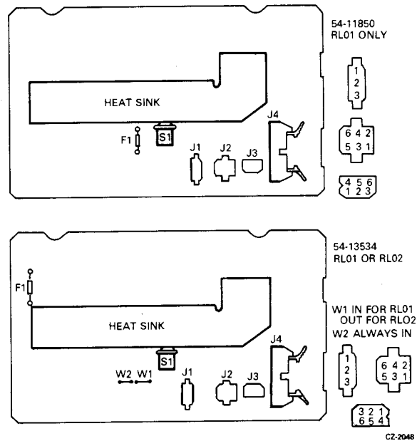
Figure 2-12 DC Servo Module Layout — Bottom View
