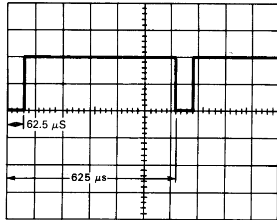
Figure 9-2 Sector Pulse Timing
