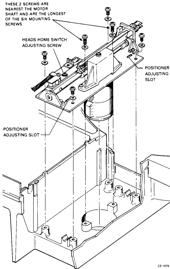
Figure 9-5 Positioner Assembly
