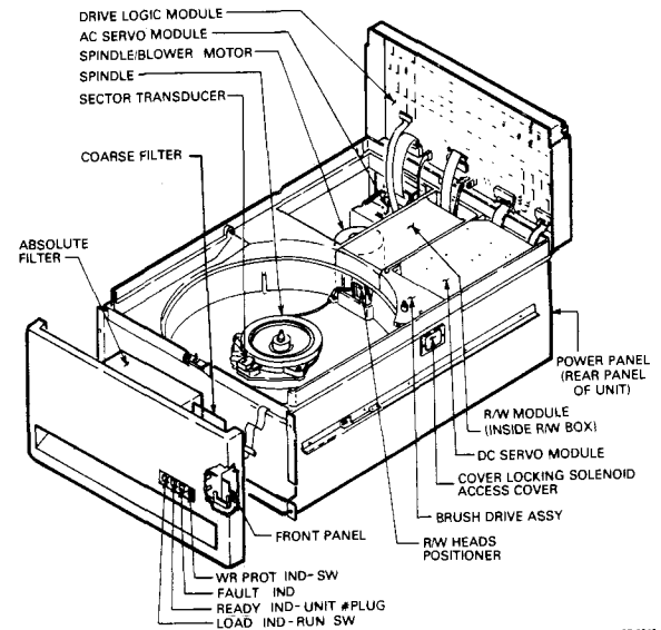
Figure 2-7 Physical Location of FRUs
