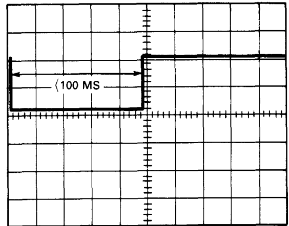
Figure 9-14 Access Time Check (255 or 511 Track Seek)
