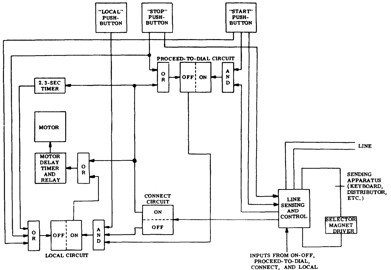
Figure 7 - Circuit Interconnections
