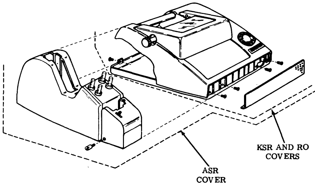
Figure 1 - Set Covers
