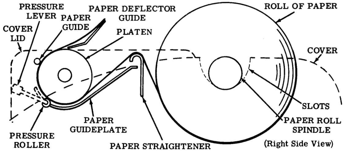
Figure 12 - Paper Threading — Friction Feed
