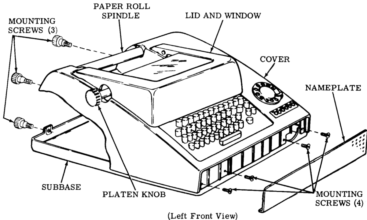
Figure 2 - Cover Mounting
