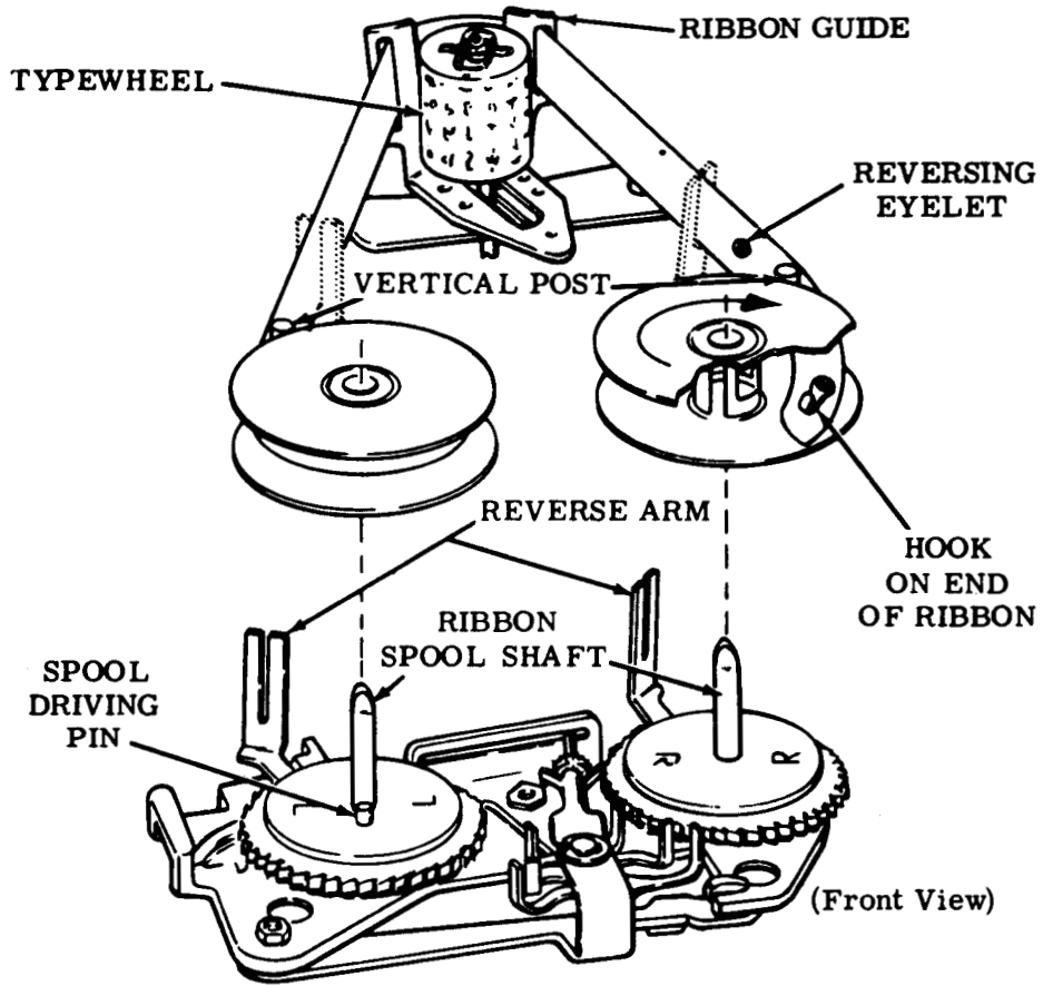
Figure 11 - Ribbon Threading
