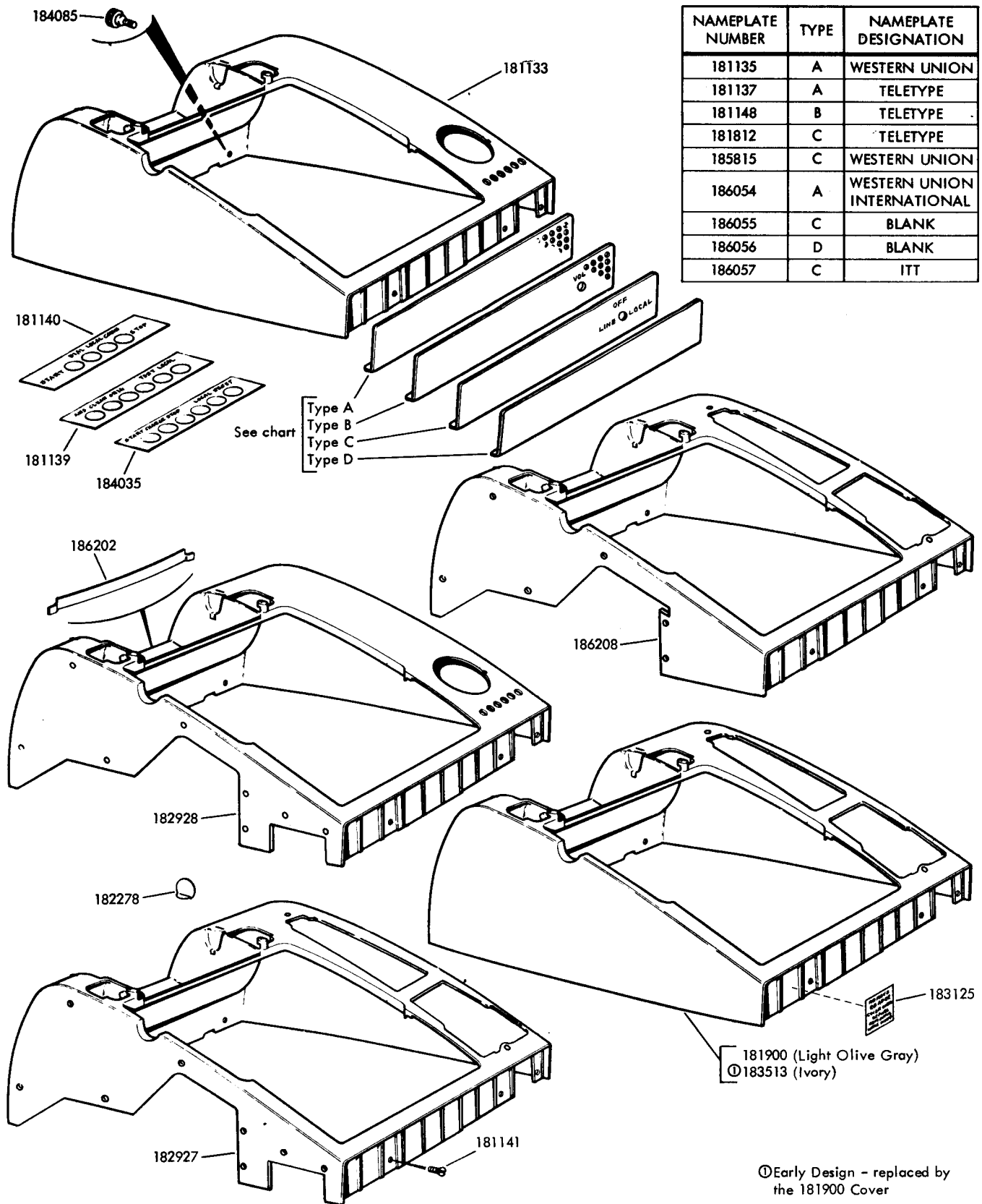
FIGURE 1. PRINTER COVERS
