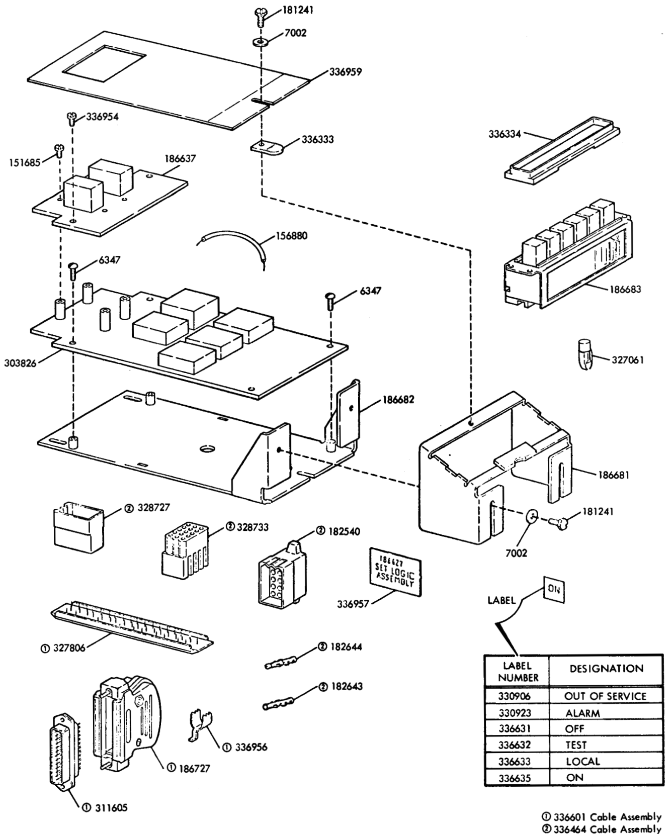
FIGURE 12. 186627 SET INTERFACE LOGIC ASSEMBLY
