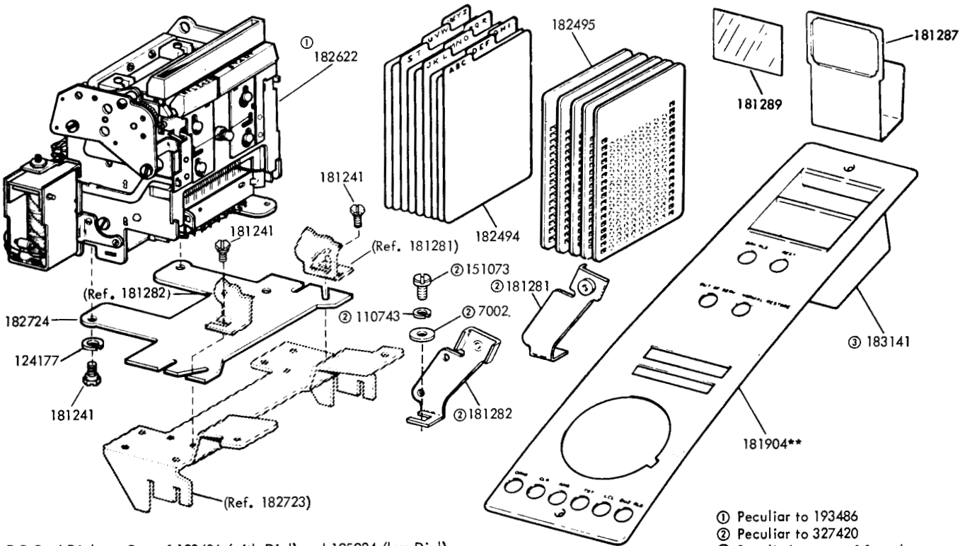
DC Card Dial Part of 193486 (with Dial) and 195924 (less Dial) Modification Kits (Specification 50164S) and 327420 (less Dial) Modification Kit (Specification 501565)
