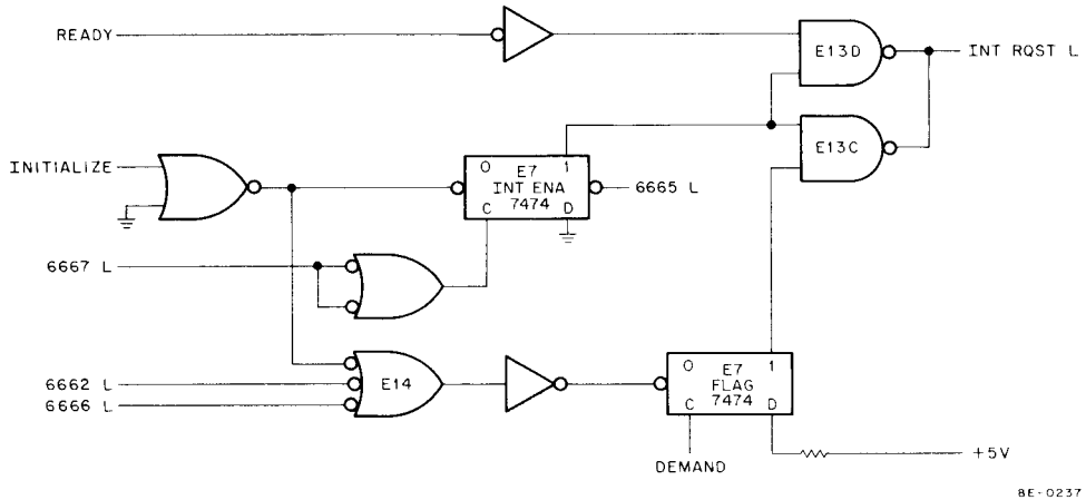
Figure 4-4 Interrupt Logic
