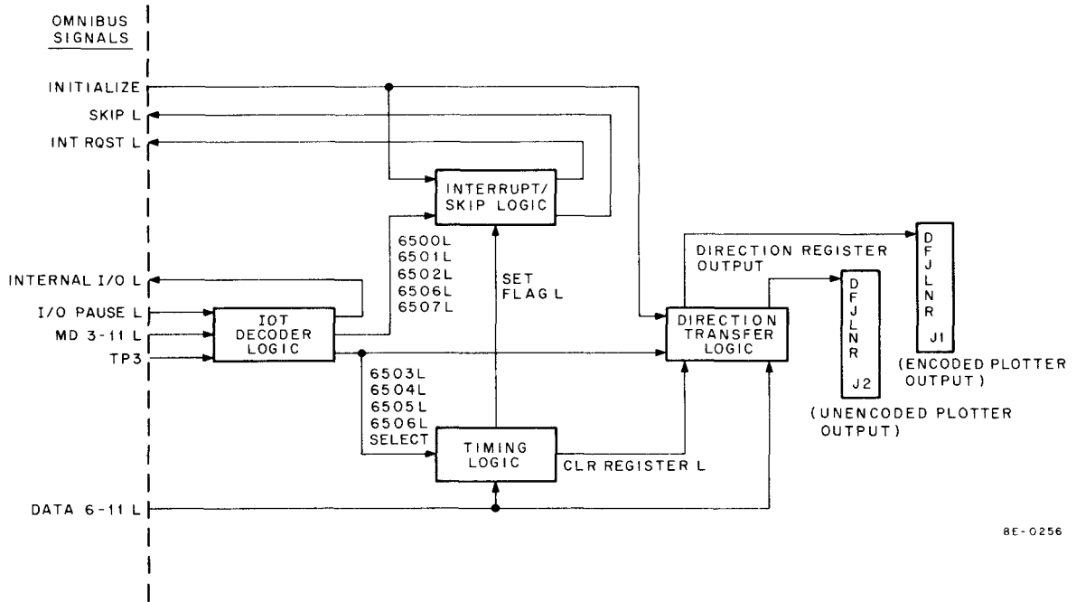
Figure 3-1 XY8-E Block Diagram
