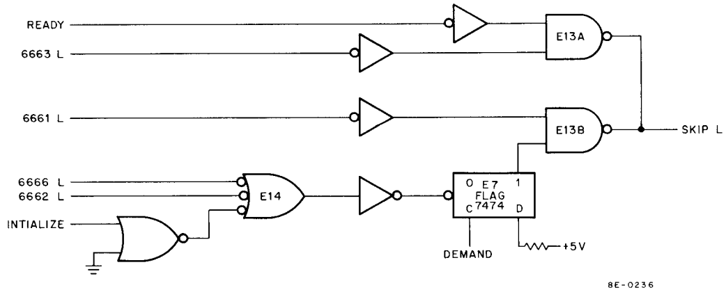
Figure 4-5 Skip Logic
