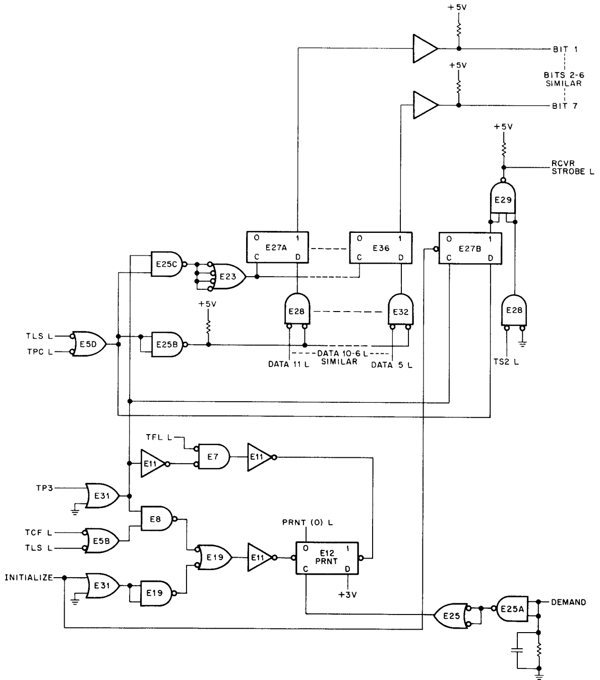
Figure 1-3 Printer Receive Logic
