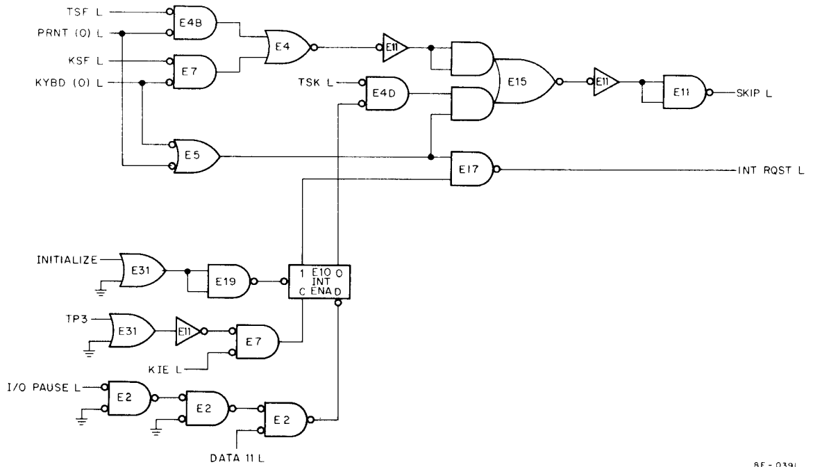
Figure 1-7 INT/Skip Logic
