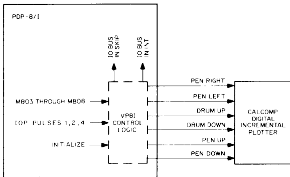
Figure 1 VP8/I Block Diagram
