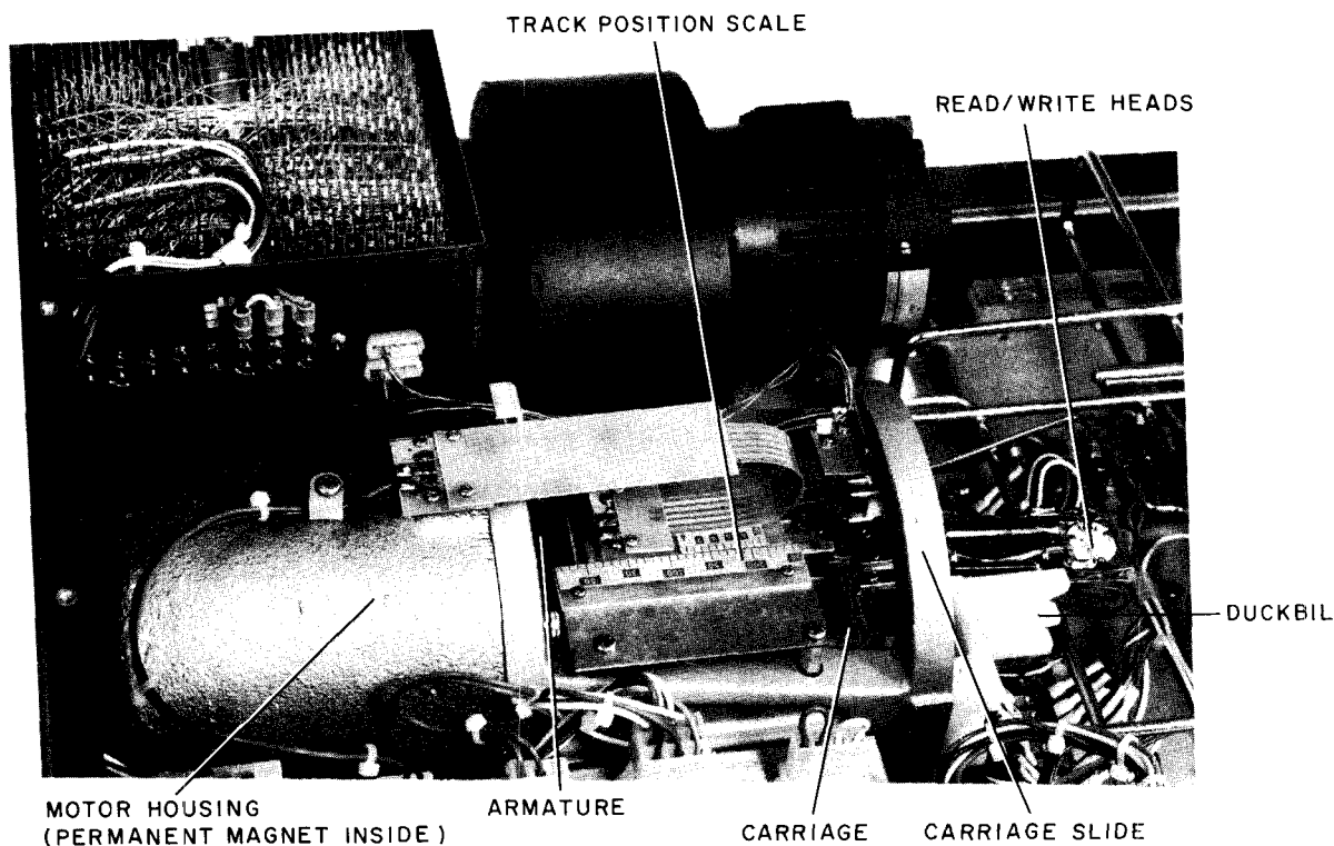
Figure 1-4 Linear Positioner
