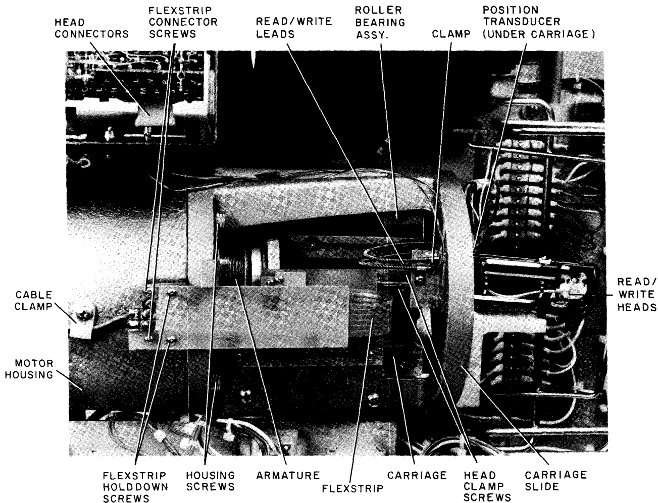
Figure 5-5 Carriage Removal
