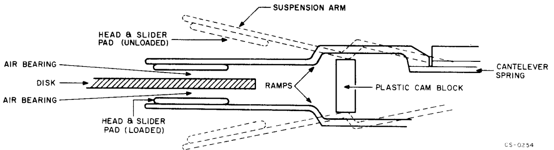
Figure 4-6 Head Loading
