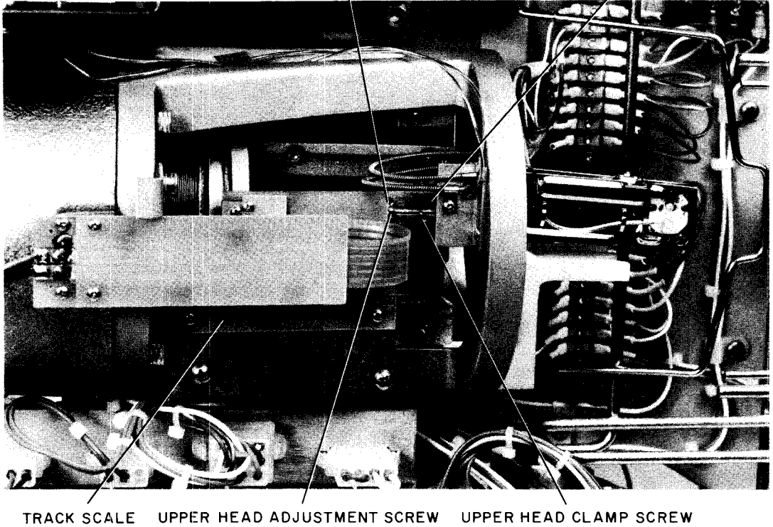
Figure 5-11 Read/Write Head Adjustments
