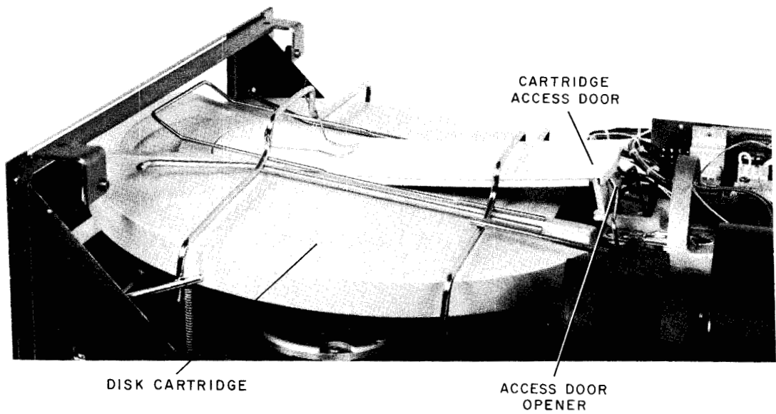
b. Cartridge Inserted
