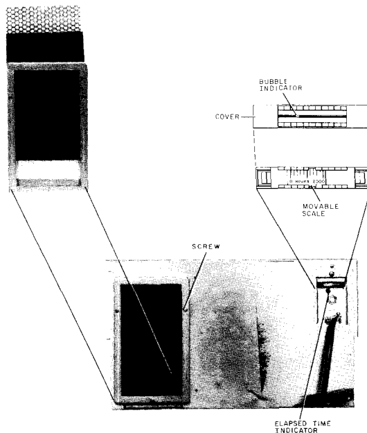
Figure 5-1 Prefilter Removal
