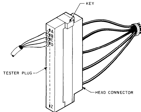
Figure 4-4 Skew Tester to Head Cable Connection
