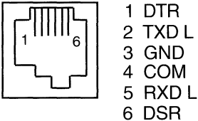
Figure B-2 Comm2 and Comm3—MMJ Ports
