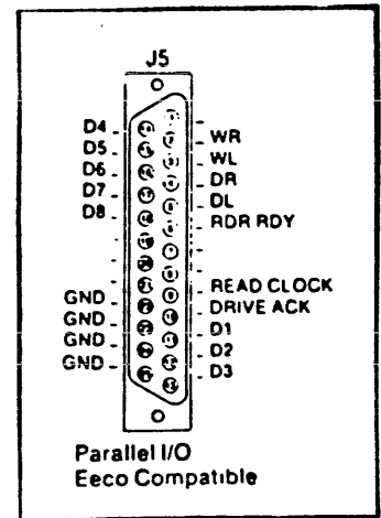
DB25S (female)
