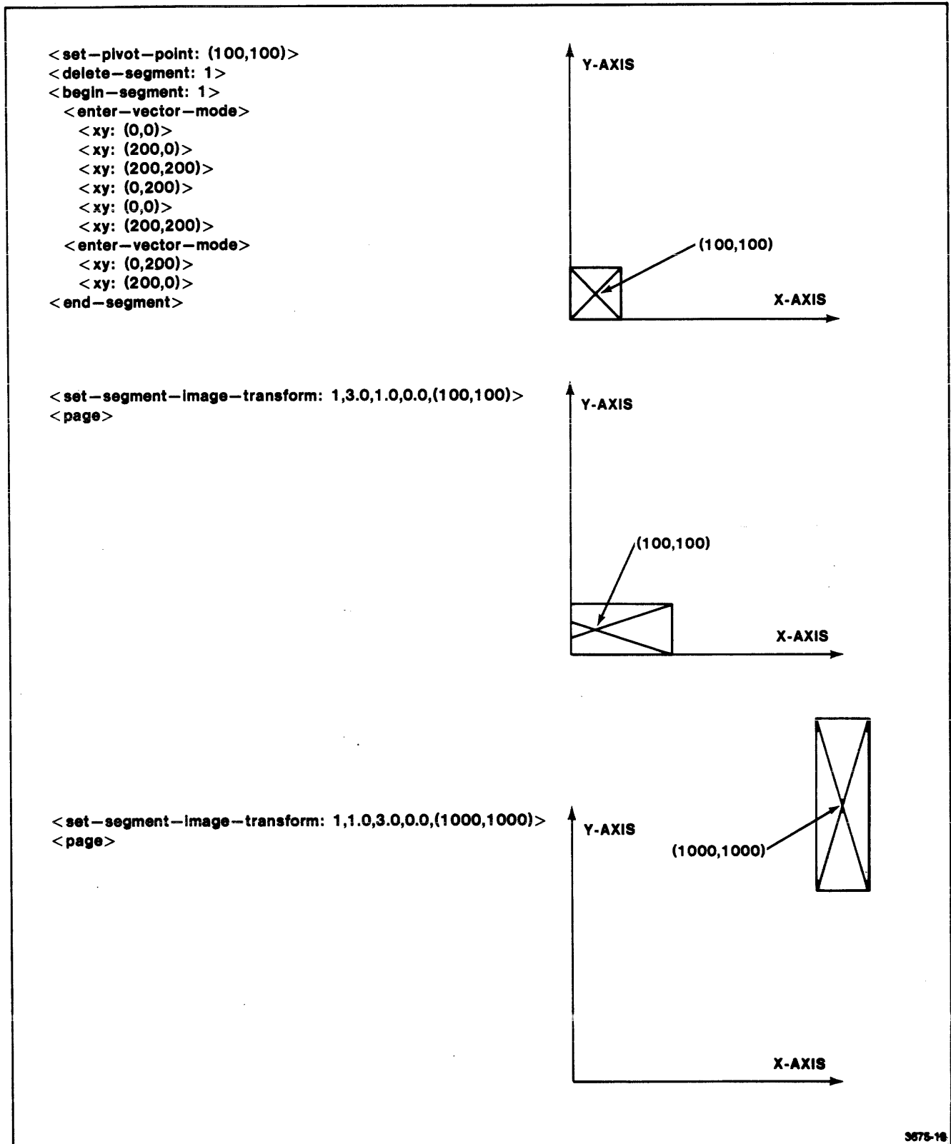
Figure 6-5. Examples of <Set-Segment-Image-Transform> Command.
