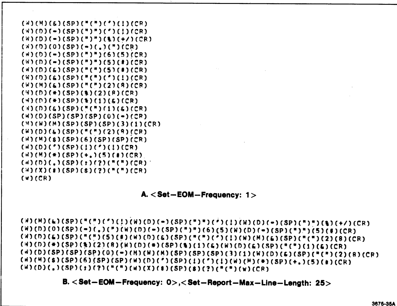
Figure 9-1. Controlling the Format of a <GIN-Report-Sequence>.
