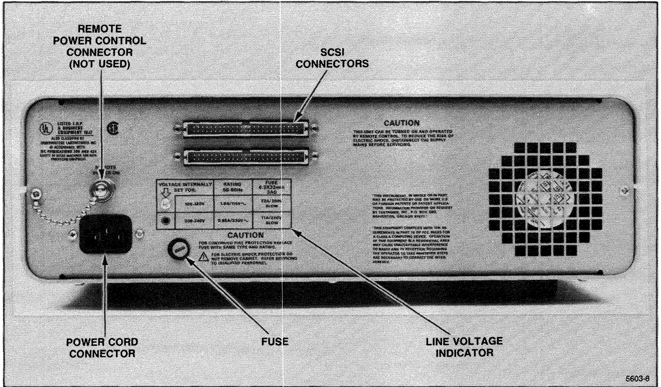
Figure 1-8. Rear of MSU.
