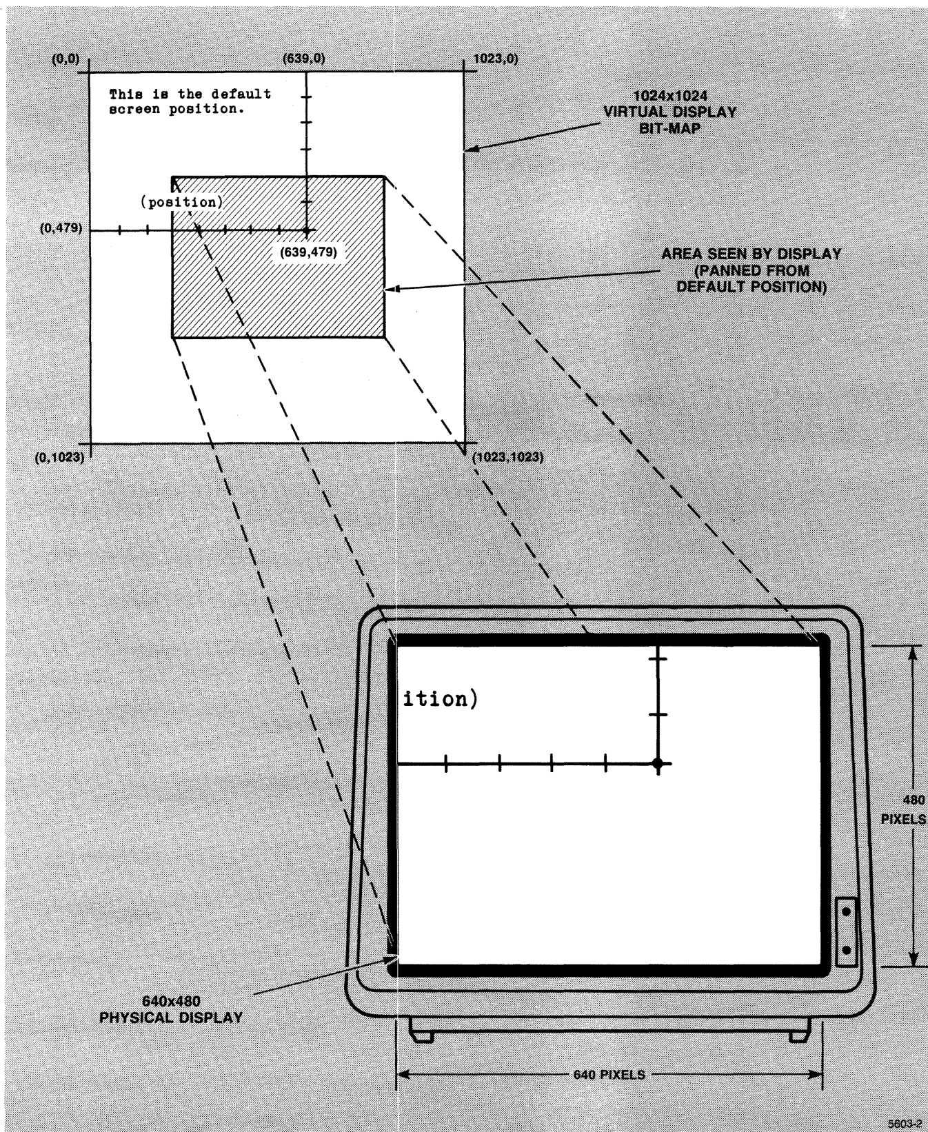
Figure 1-2. 640 X 480 Window Into 1024 X 1024 Bit-Map.
