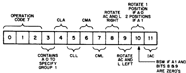
Figure 3-4 Group 1 Operate Instruction Bit Assignments
