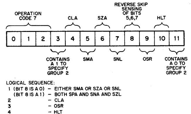
Figure 3-5 Group 2 Operate Instruction Bit Assignments
