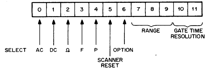
Figure 7-24 Control Word 1 (from Computer)
