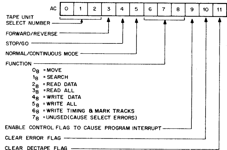
Figure 7-21 Status Register A Bit Assignments
