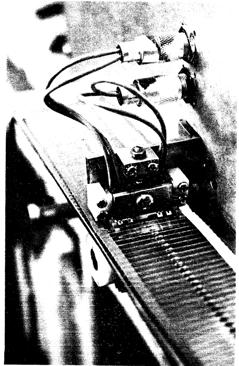
All incoming components are 100% tested. Here, diodes are being tested automatically.
