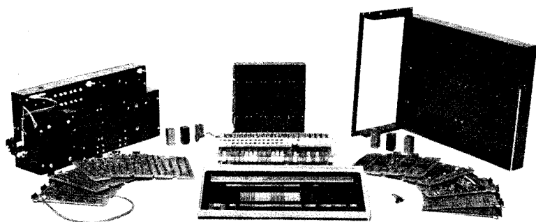
PDP-8/E System Assembly —After testing all the various components of a PDP-8/E Computer, the components are carefully assembled. This photo shows all of the components for a basic 4K Computer arranged to illustrate how modular the 8/E is and how spare parts can easily be the key to zero downtime.
