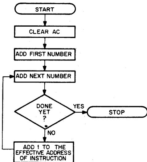
Figure 4-8 Address Modification
