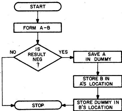
Figure 4-9 Conditional Skip
