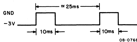
Figure 6-2 10 ms Change Reader Delay Waveform
