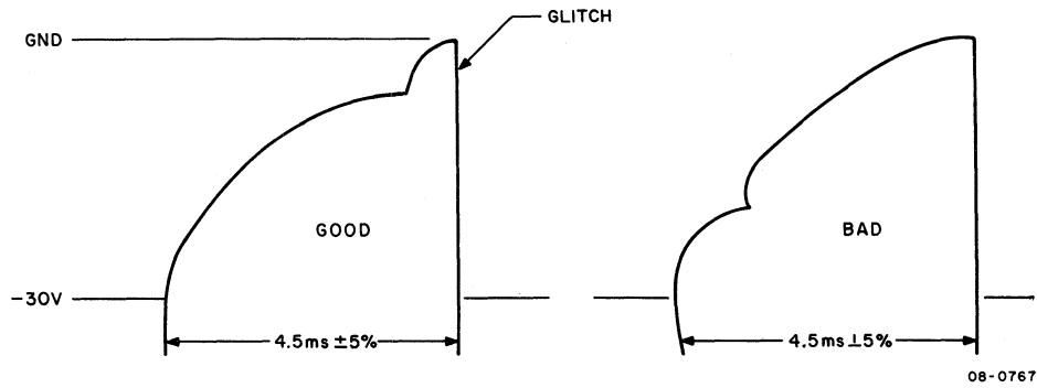
Figure 6-12 Punch Solenoid Waveform
