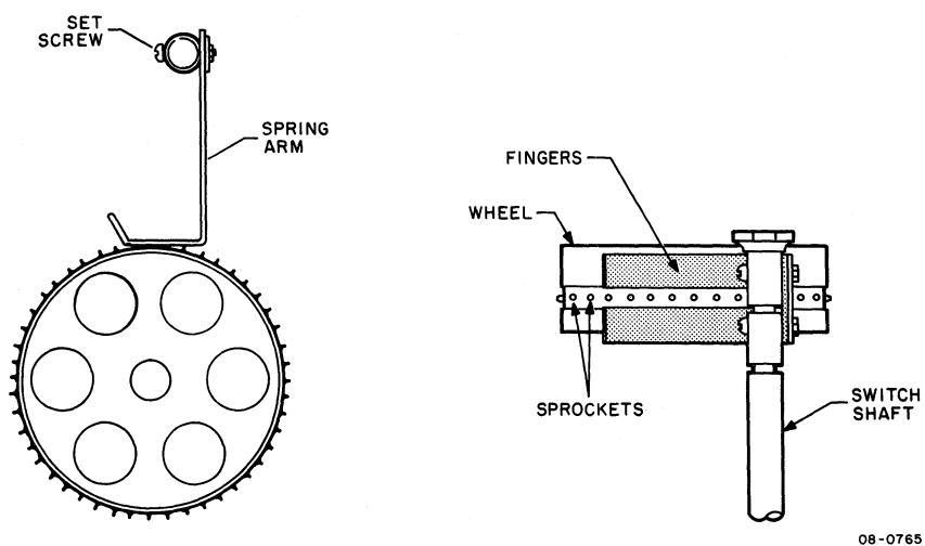
Figure 6-10 Spring Arm Adjustment
